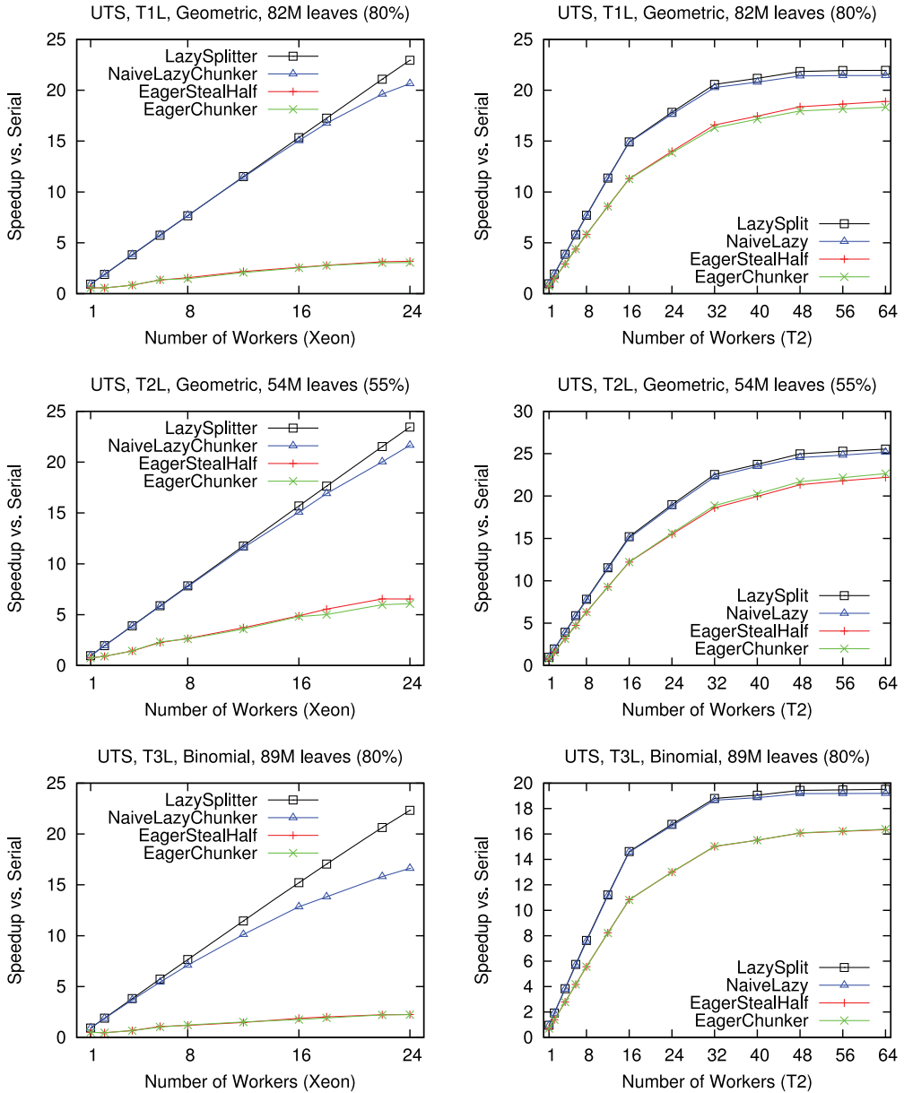
Fig. 16. UTS speedup results on Xeon and T2 (original PThreads implementation).
