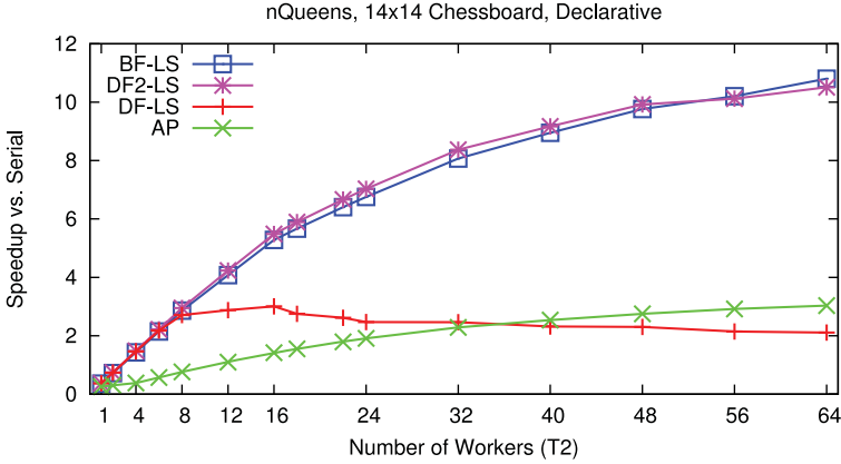
Fig. 7. Performance scaling of schedulers on T2 (nQueens).
