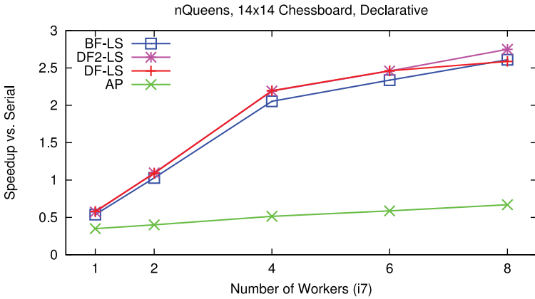
Fig. 9. Performance scaling of schedulers on i7 (nQueens).
