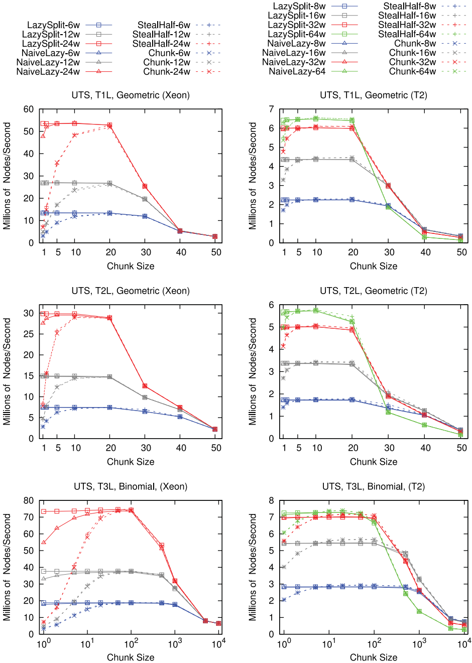
Fig. 17. UTS sensitivity results on Xeon and T2 (original PThreads implementation).
