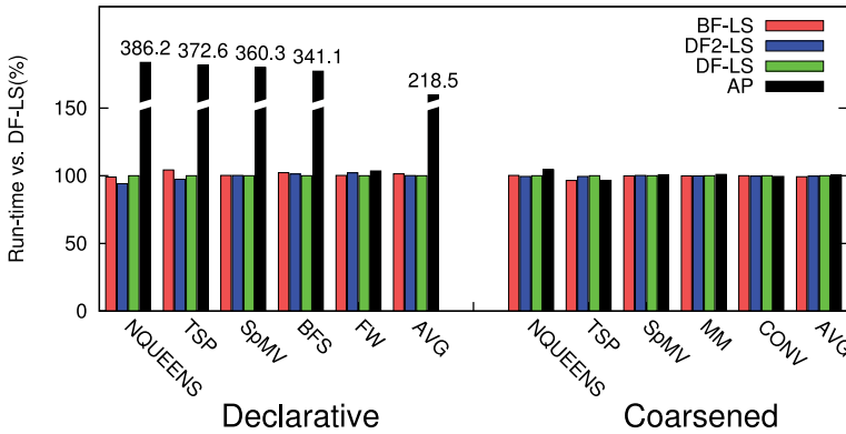
Fig. 10. Benchmarks on the i7 using all eight workers.
