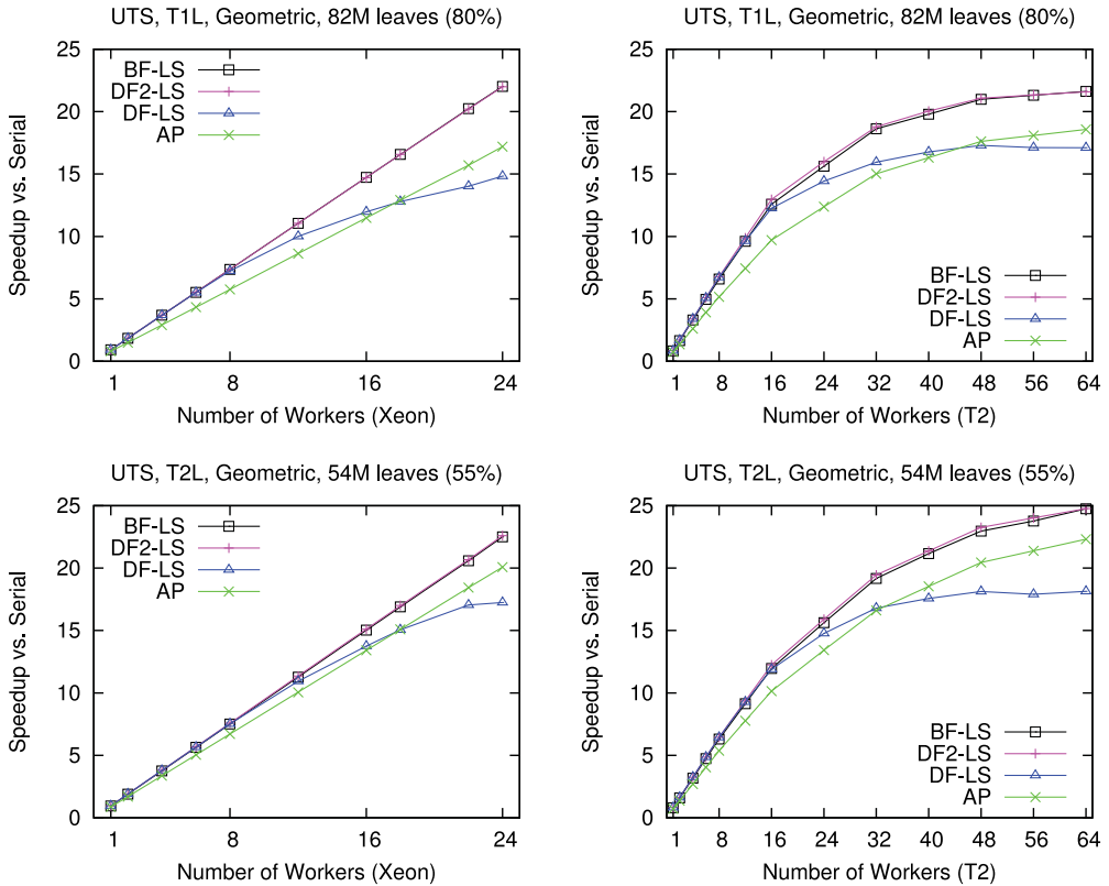
Fig. 18. UTS Speedup results on Xeon and T2 (TBB Implementation).
