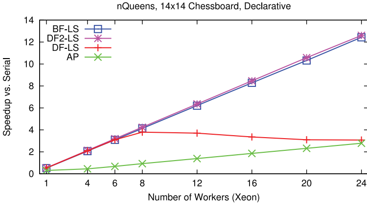
Fig. 8. Performance scaling of schedulers on Xeon (nQueens).
