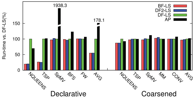
Fig. 14. Benchmarks on the T2 using all 64 workers.
