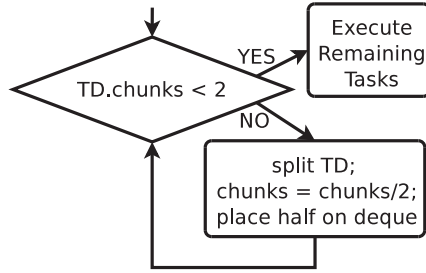
Fig. 2. Processing a task descriptor with auto-partitioner.
