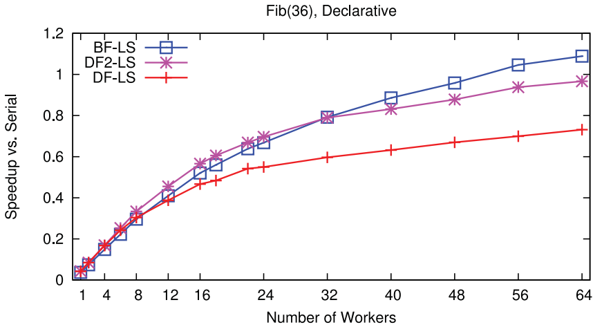
Fig. 15. Performance scaling of schedulers on T2 (Fib(36)).
